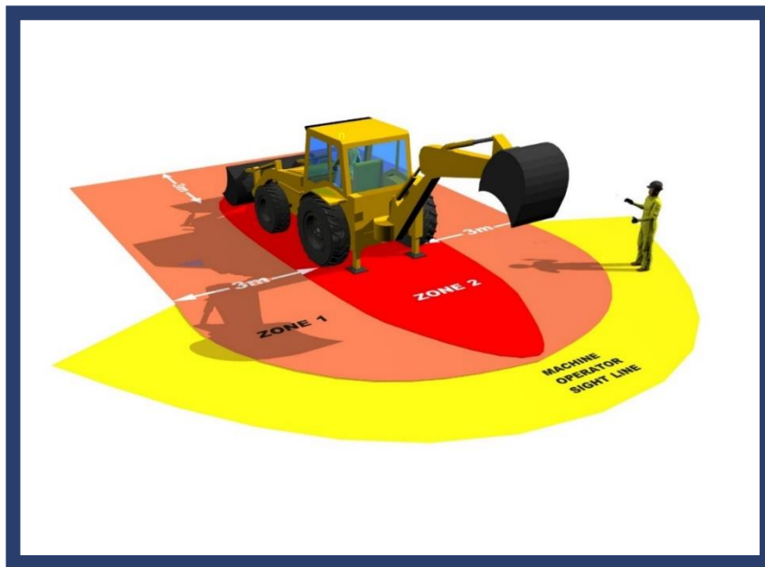
180° excavator
